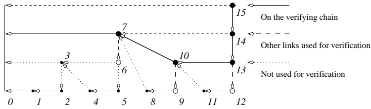
Fig. 3. The time-stamp of X_{10} in the proposed system.
