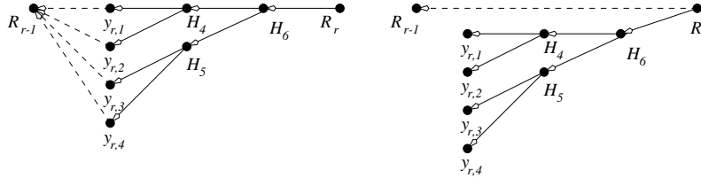
Fig. 1. An example of the time-stamp for round r by the schemes presented in [BdM91] (left) and [BHS92] (right).
